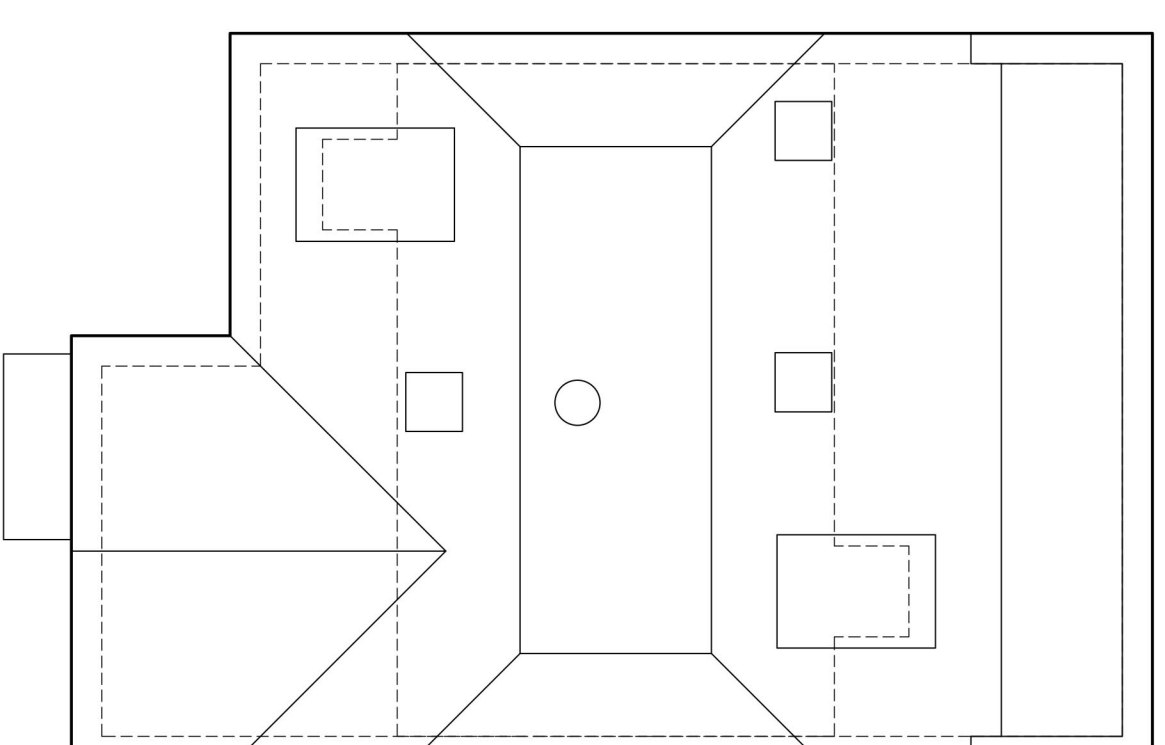
Roof Plan
