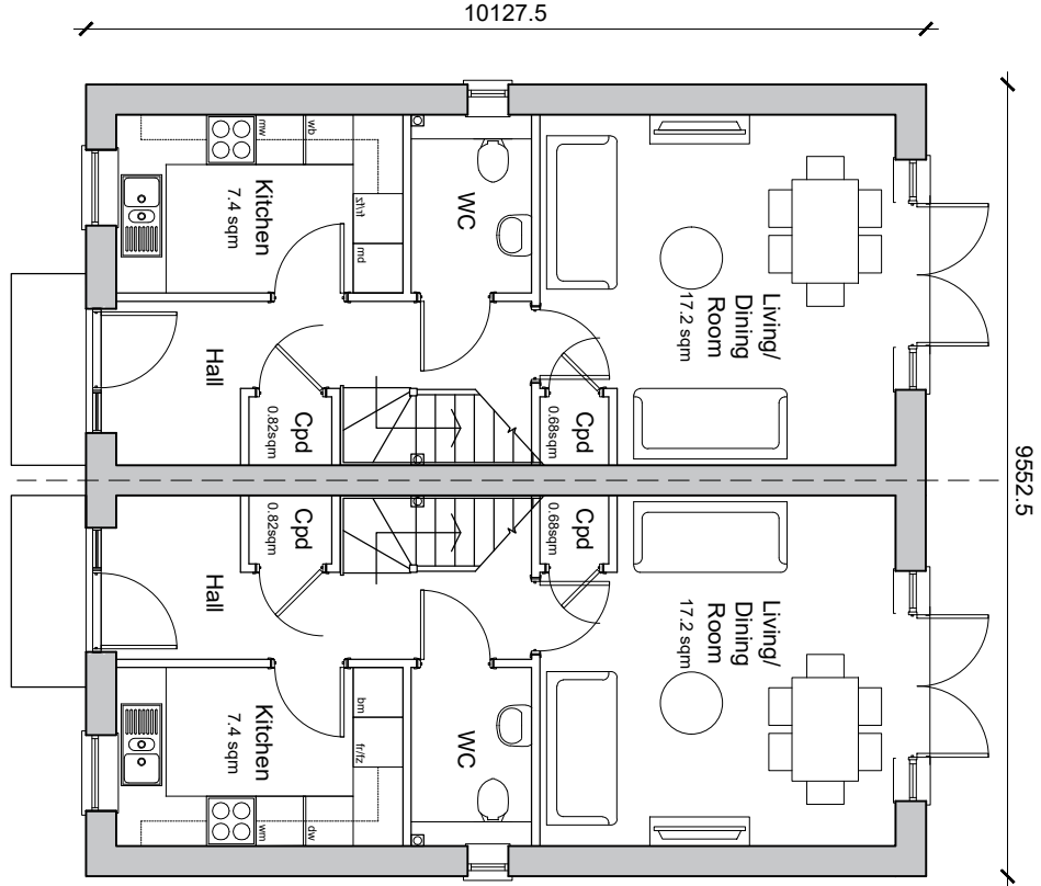
Ground Floor Plan 2 Bedrooms & Pension House 75-84 High Street, Brighton, BN1 1JL Plot 31-32, 35-36, 39-40, 66-68, 67-68 Plot 31-32, 35-36, 39-40, 66-68, 67-68
