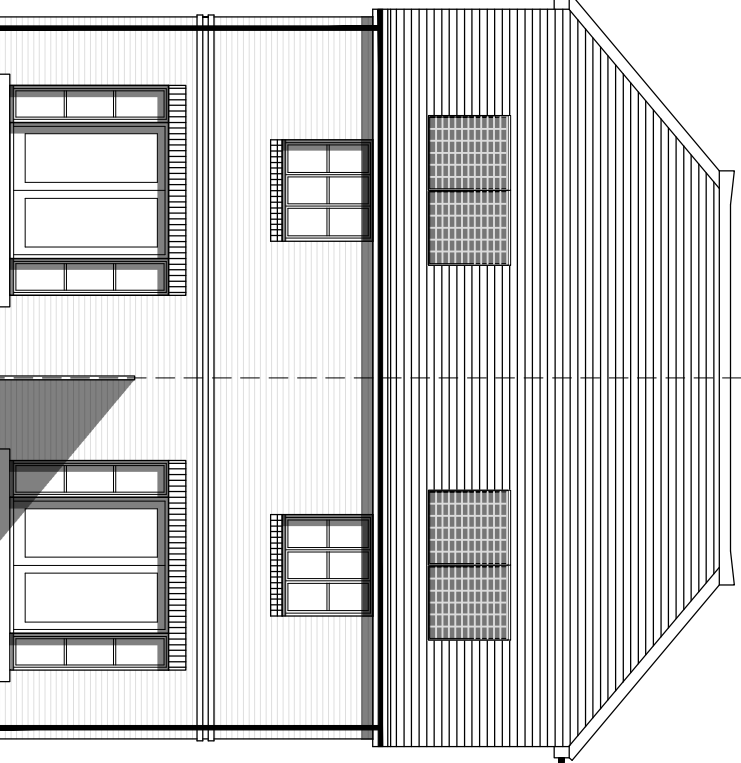
Rear Elevation
