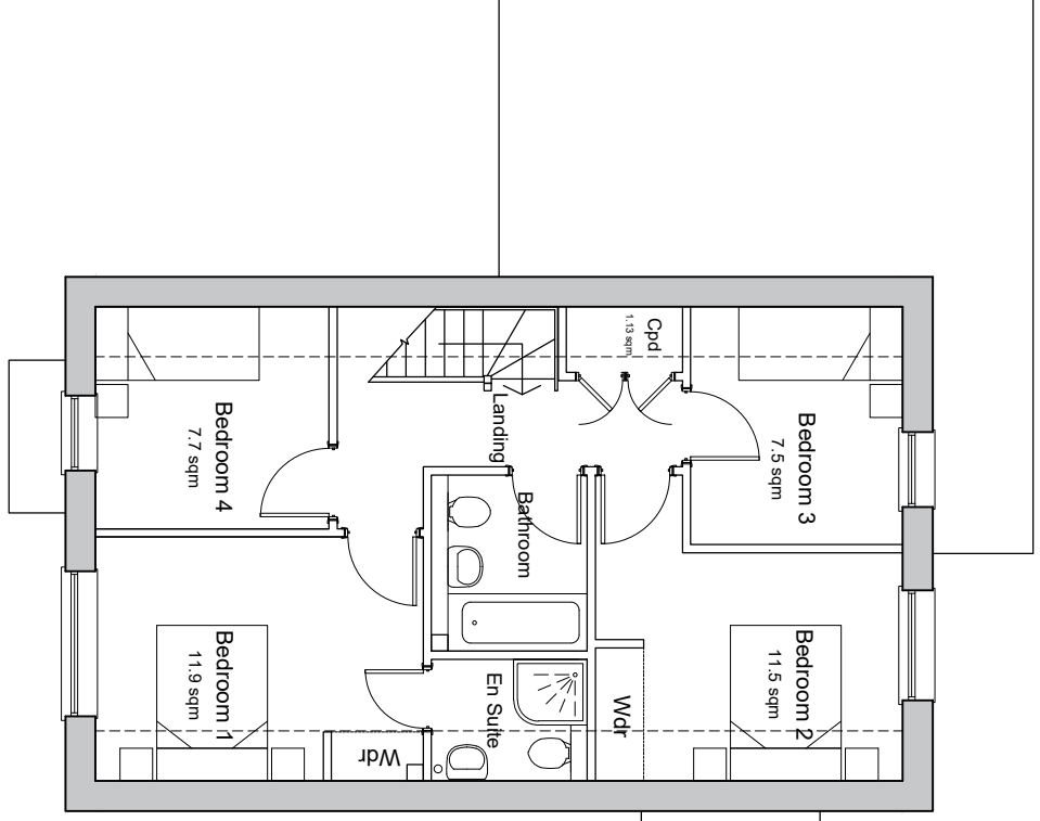
First Floor Plan Pld 02
