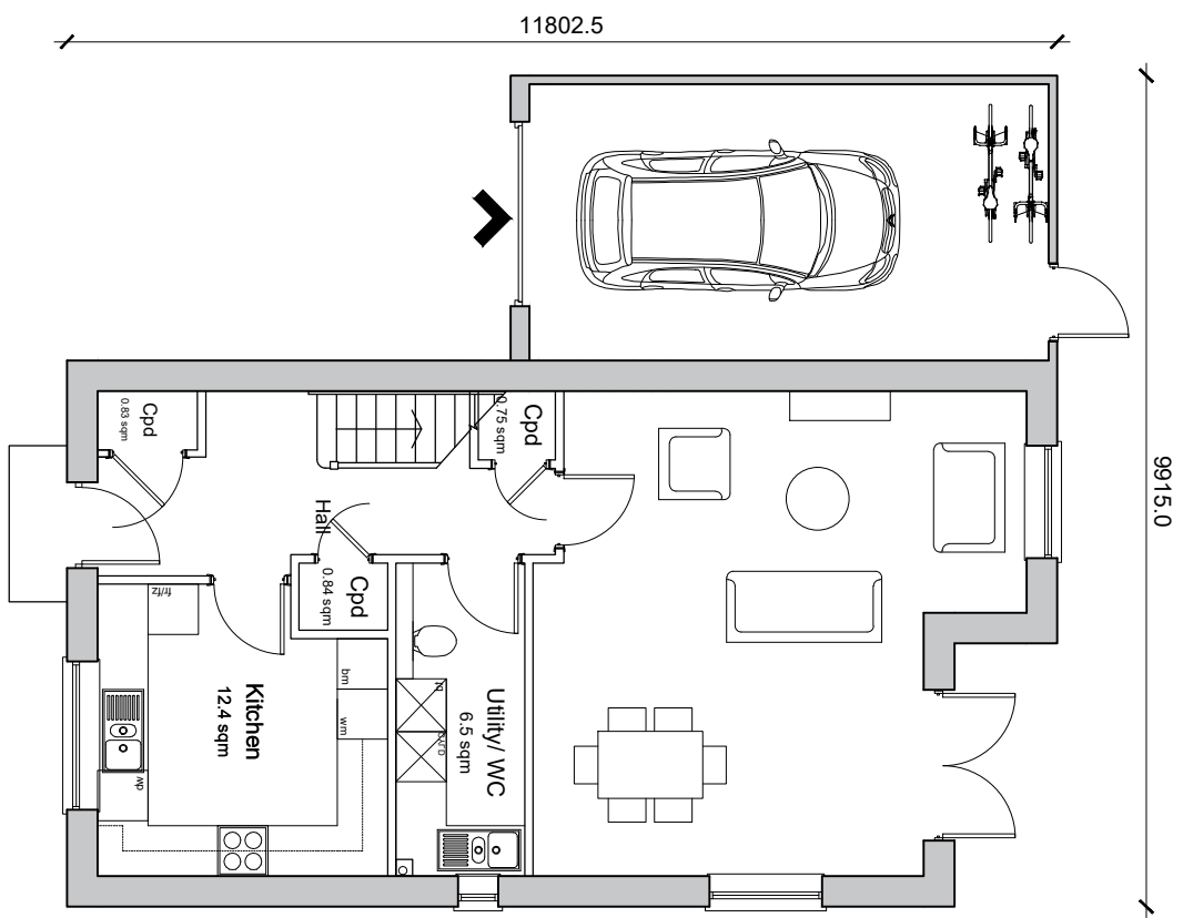
Ground Floor Plan Pld 01 4-Bedroom 5-Person House 117.00sqm / 1255sqf GFA, 34.7sqm Wet Area Architectural drawings produced in accordance with Building Regulations
