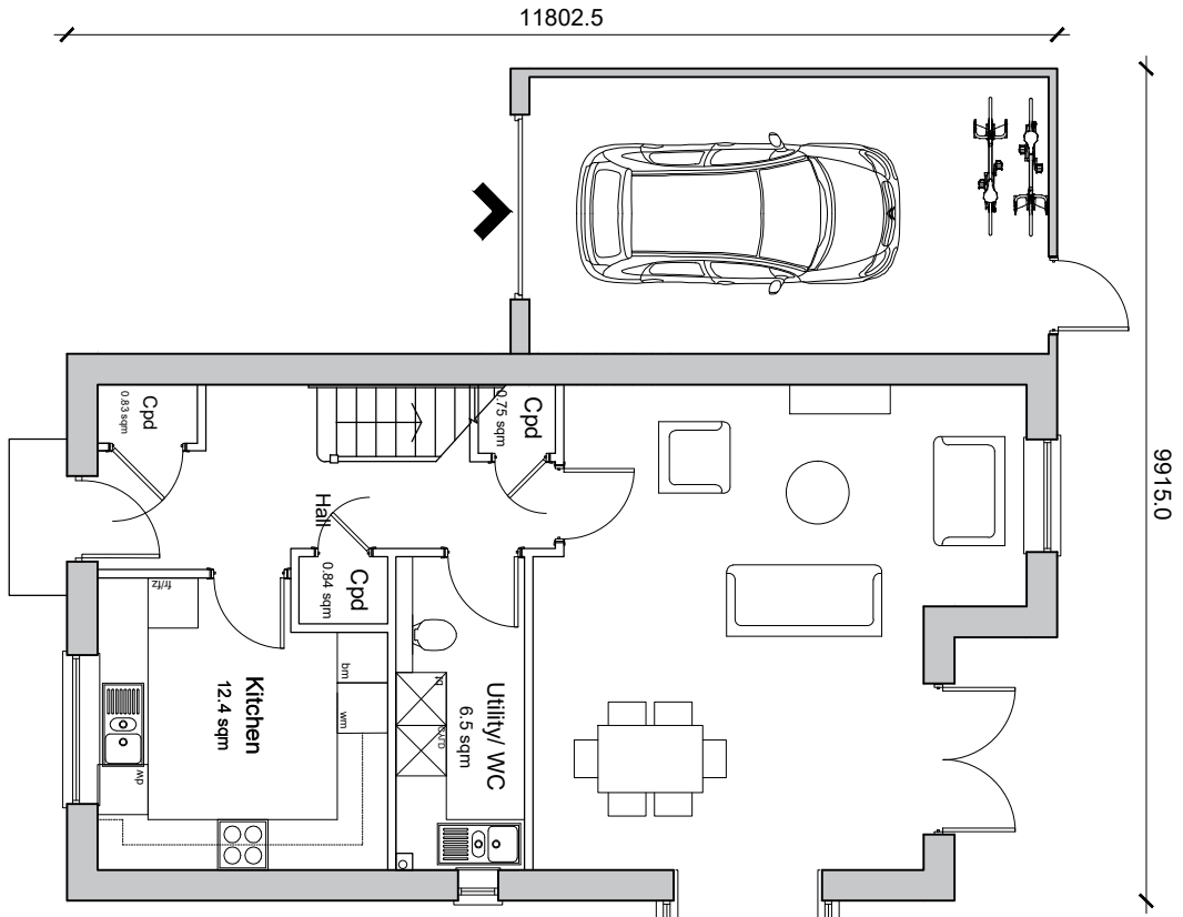
Ground Floor Plan Pld 02 4-Bedroom 5-Person House 119.5sqm / 1285sqf GFA, 34.7sqm Wet Area Architectural drawings produced in accordance with Building Regulations
