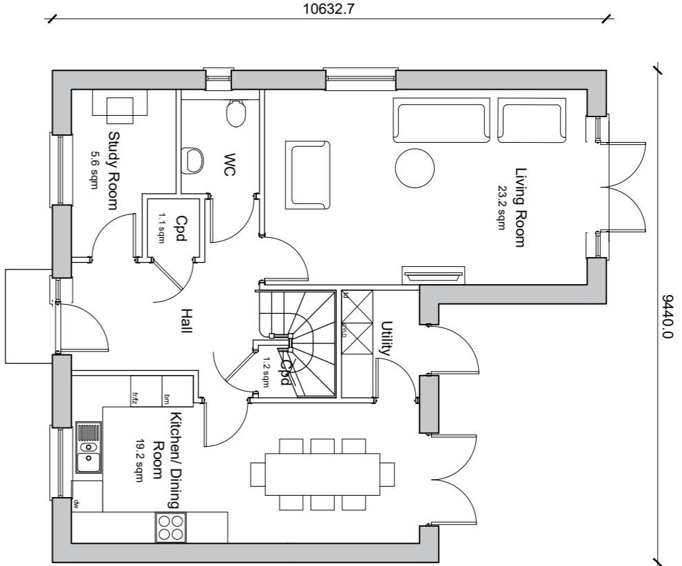
Ground Floor Plan HT08 2-Bedroom 7-Storey House 1024 sqm (11020 sqft) GFA, 36 sqm (387 sqft) GFA 1024 sqm (11020 sqft) GFA, 36 sqm (387 sqft) GFA 1024 sqm (11020 sqft) GFA, 36 sqm (387 sqft) GFA Plot 54
