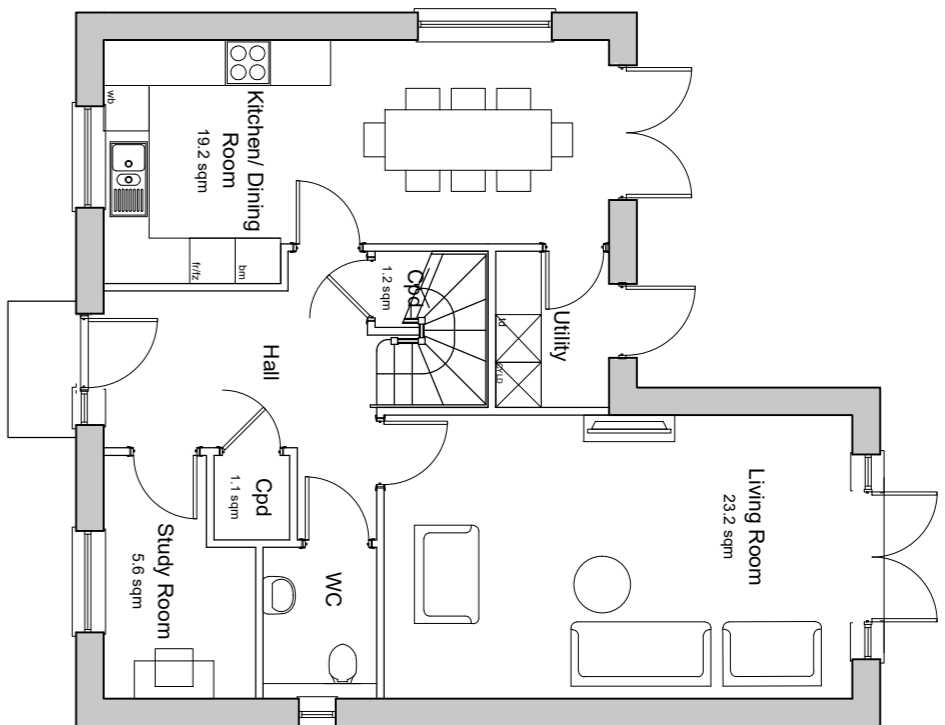
Ground Floor Plan HT08 2-Bedroom 7-Storey House 1024 sqm (11020 sqft) GFA, 36 sqm (387 sqft) GFA 1024 sqm (11020 sqft) GFA, 36 sqm (387 sqft) GFA 1024 sqm (11020 sqft) GFA, 36 sqm (387 sqft) GFA Plot 53
