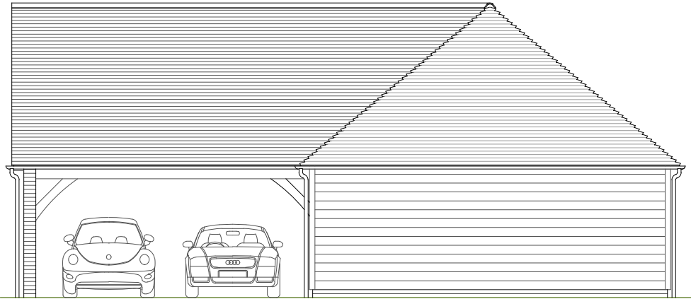
North 1:100 | PROPOSED
