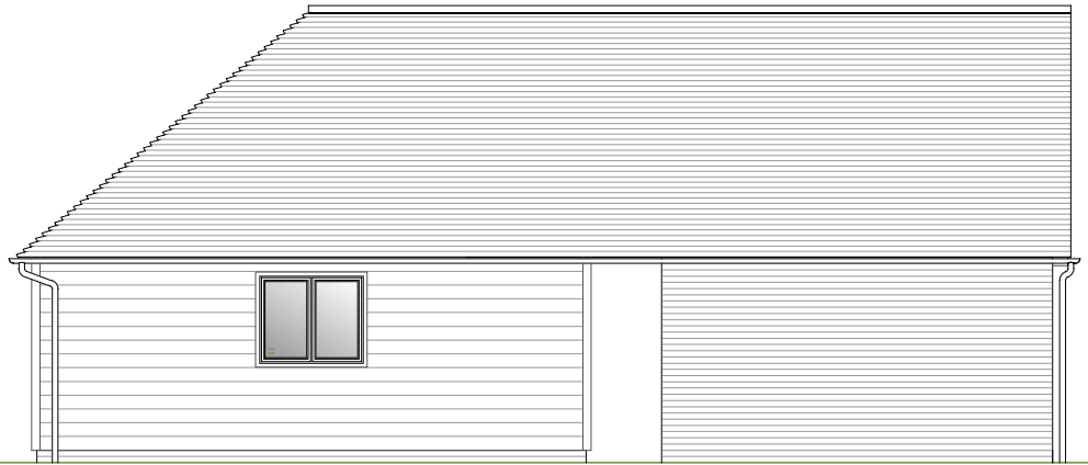
South 1:100 | PROPOSED
