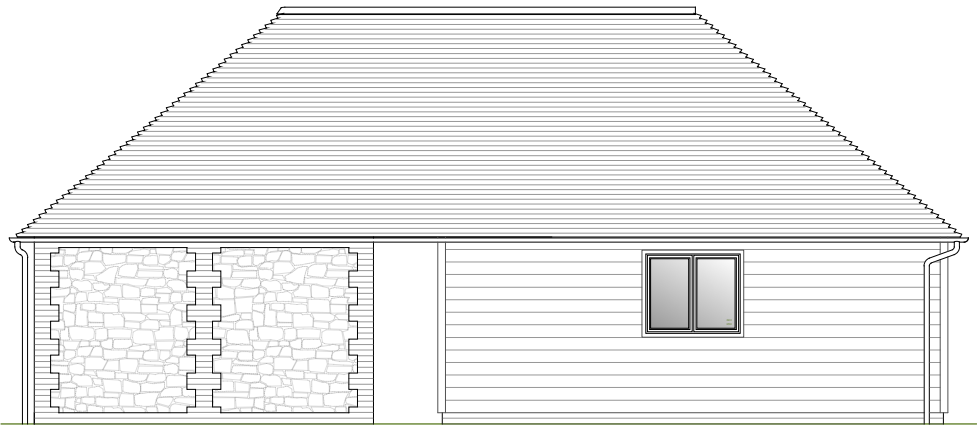
North 1:100 | PROPOSED
