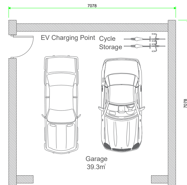
Proposed Floor Plan - Garage C
