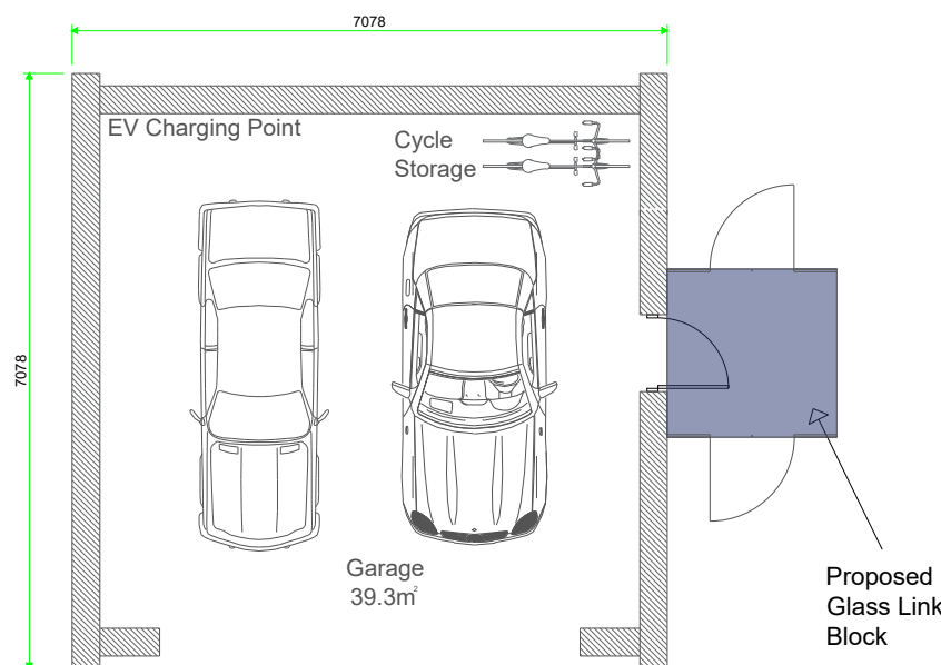
Proposed Floor Plan - Garage B
