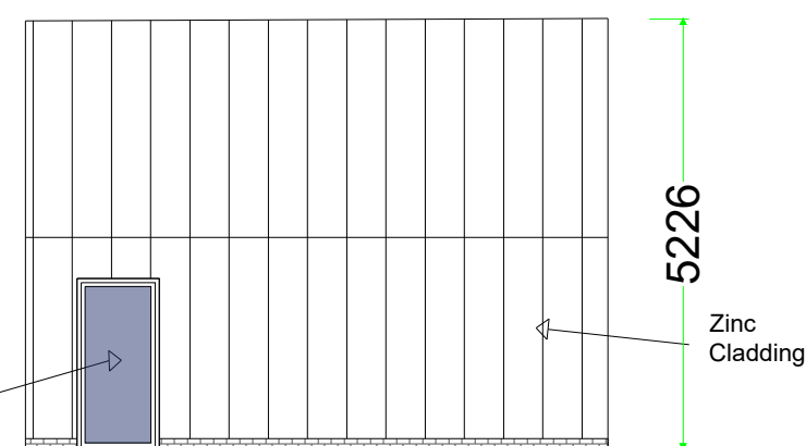
Proposed East Facing Elevation - Plot C
