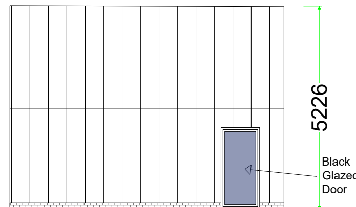
Proposed East Facing Elevation - Plot A
