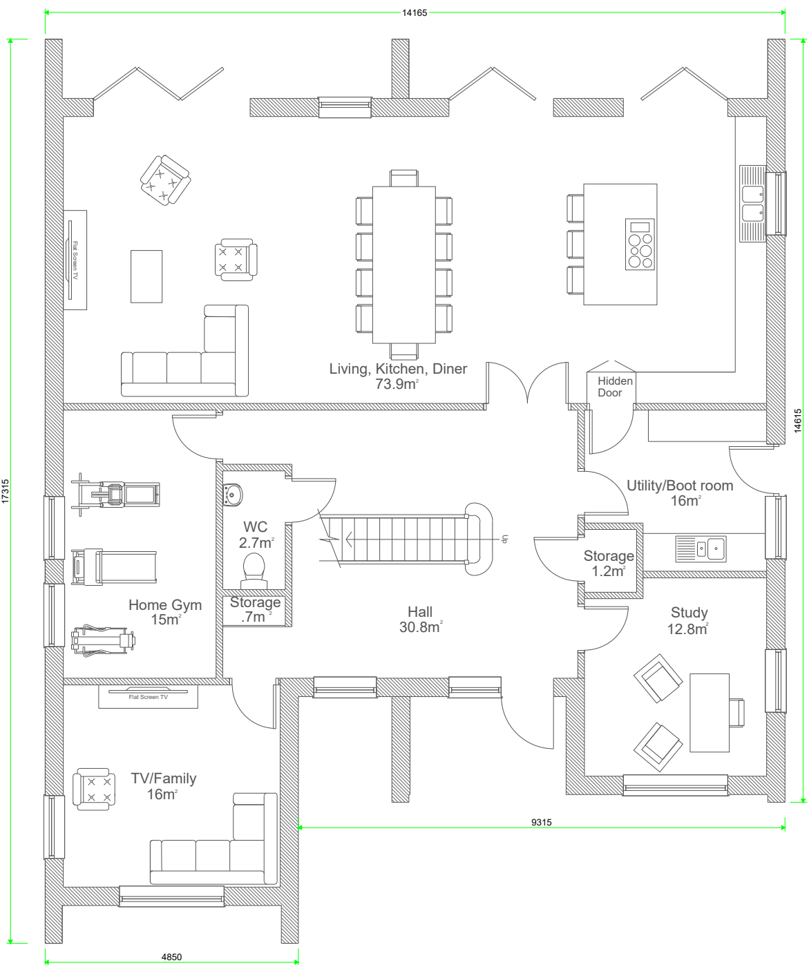
Proposed Ground Floor Plan (Plot C)
