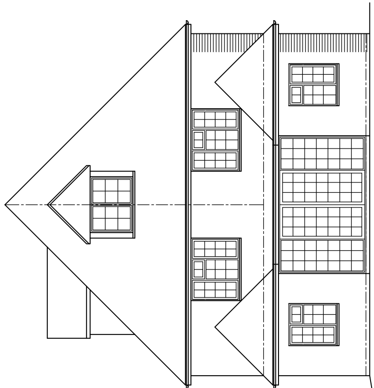
EAST ELEVATION
