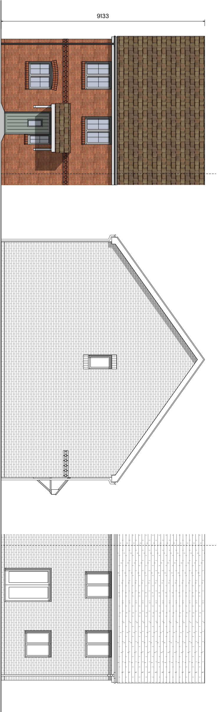
Front Elevation
