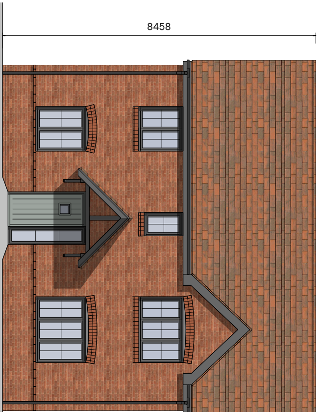
Front Elevation
