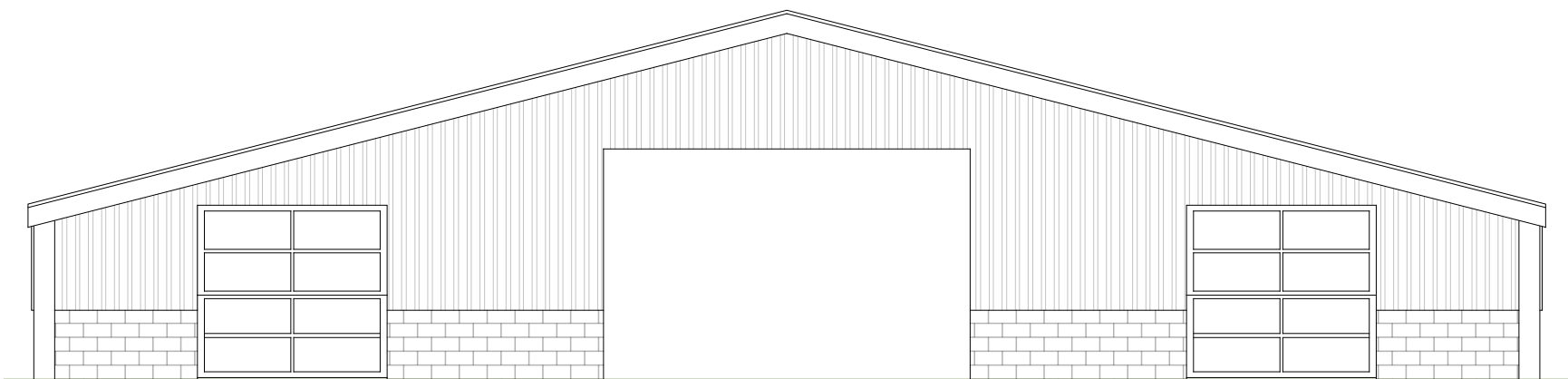
North Elevation 1:100
