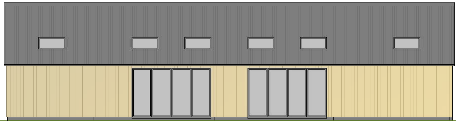
East Elevation 1:100
