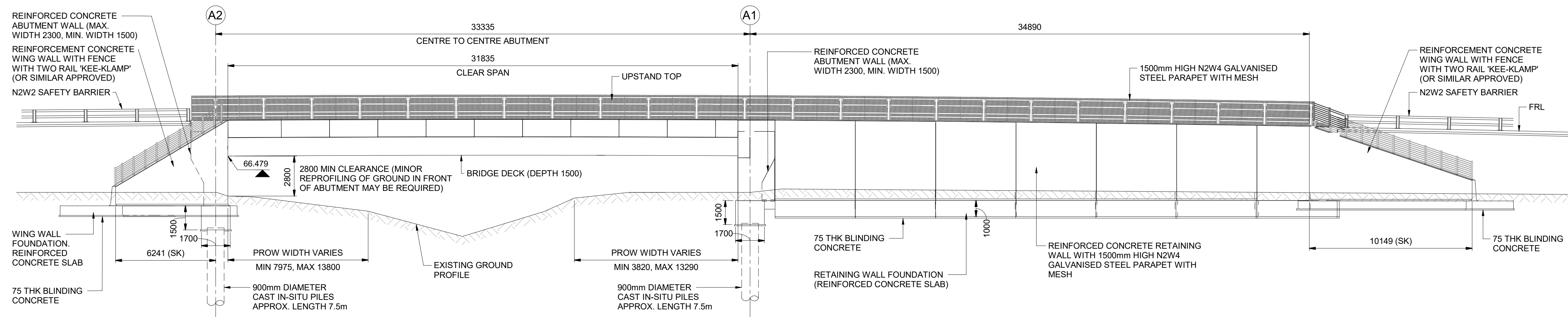
A ELEVATION A 00001 1 : 150
