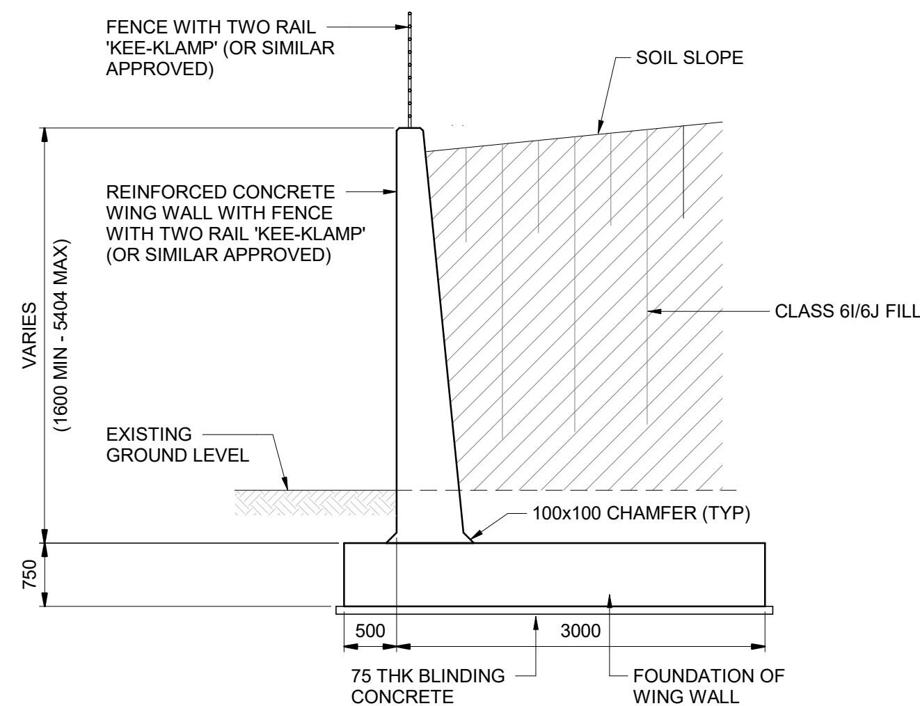
TYPICAL SECTION THROUGH WINGWALL 1 : 50
