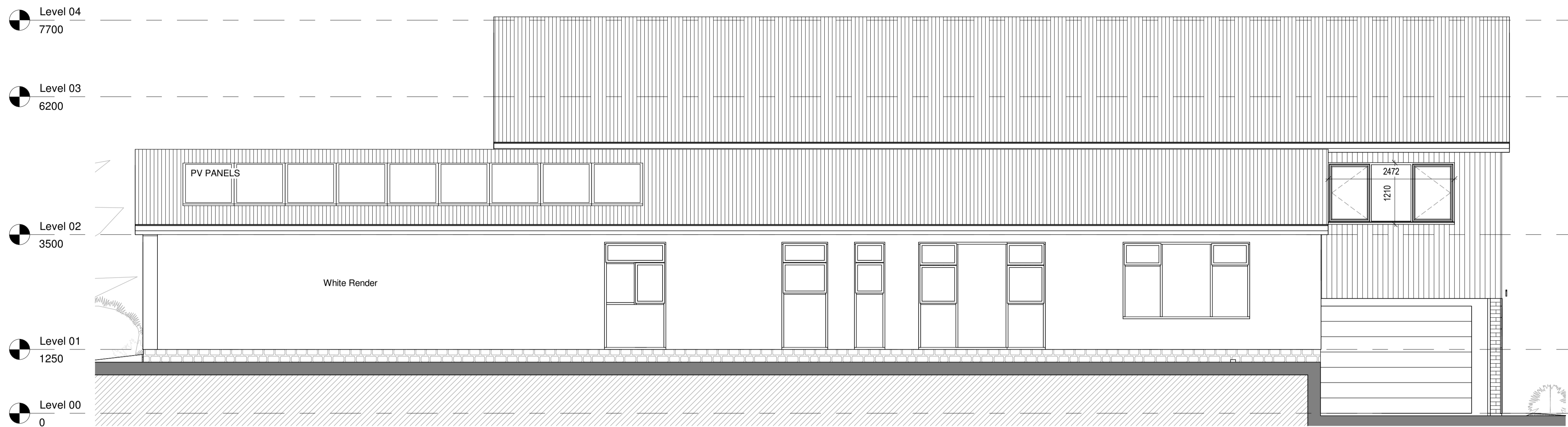
1 East Elevation - Proposed 1 : 50
