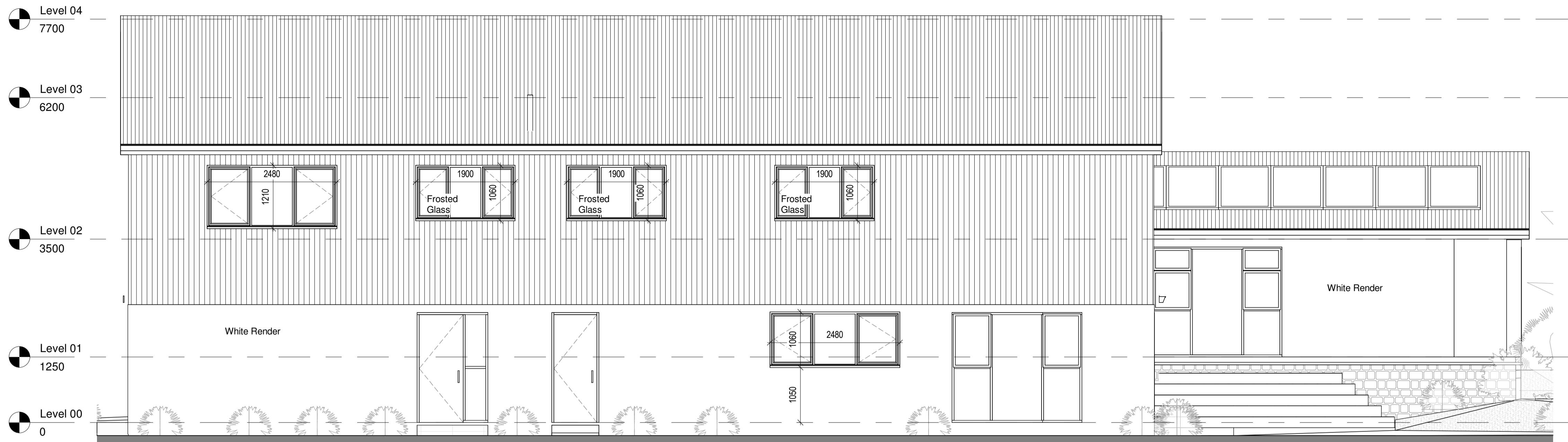
1 West Elevation - Proposed 1 : 50
