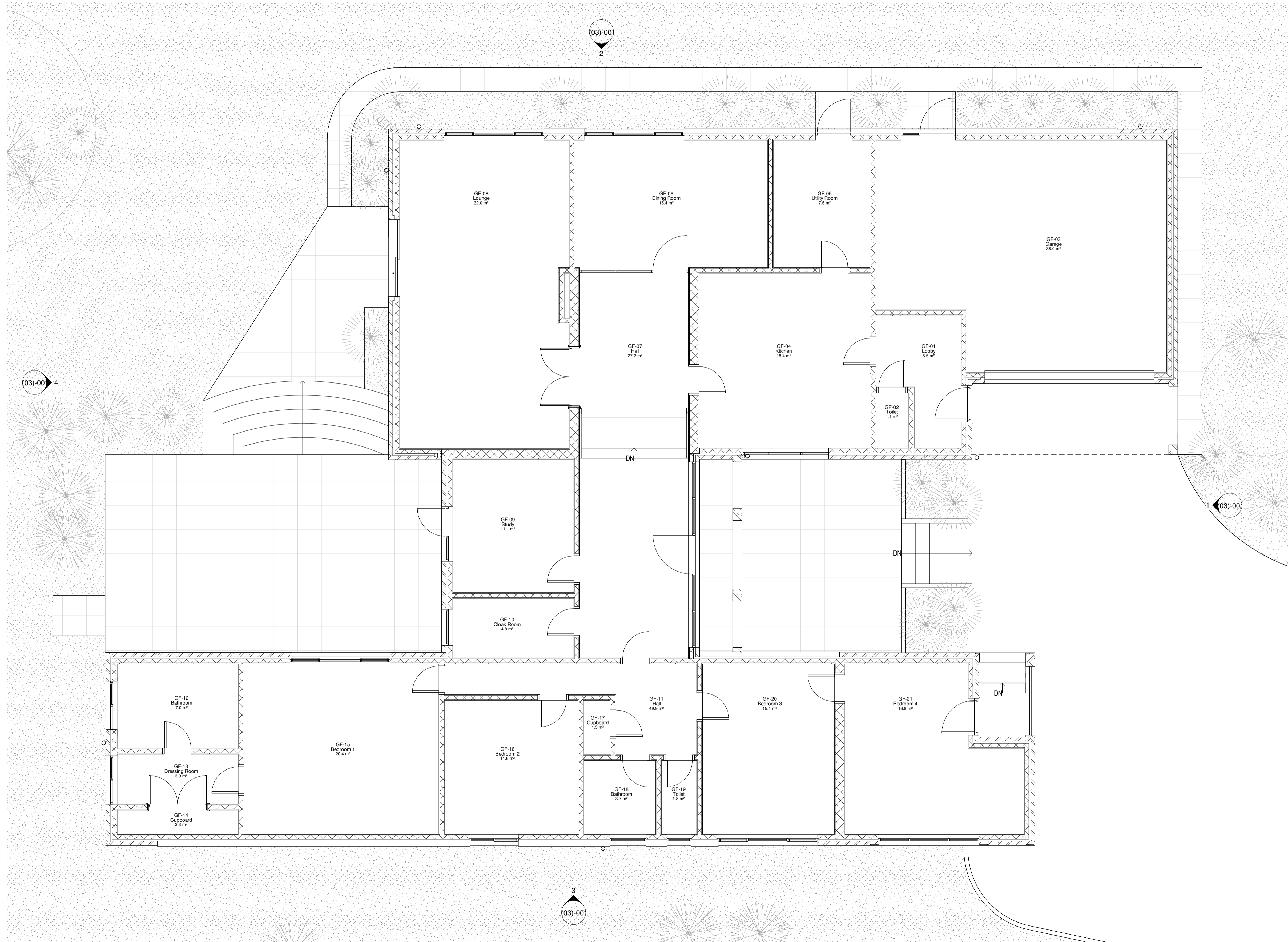
1 Ground Floor - Existing Plan 1 : 50
