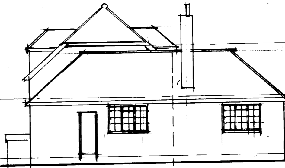
SIDE ELEVATION (W)
