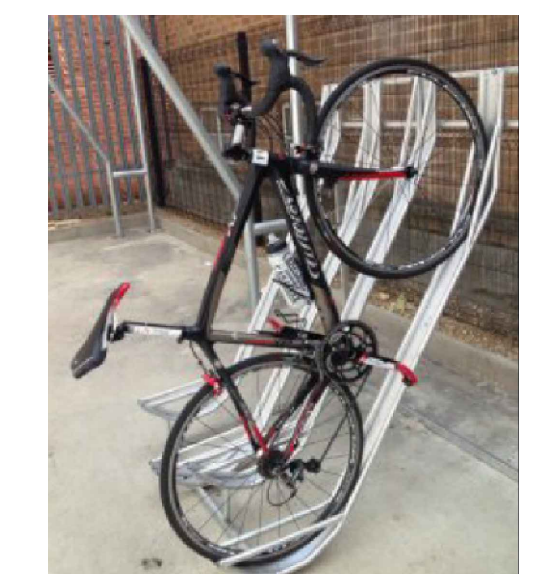
Example of a good quality semi-vertical bike rack to be provided within communal cycle stores.
