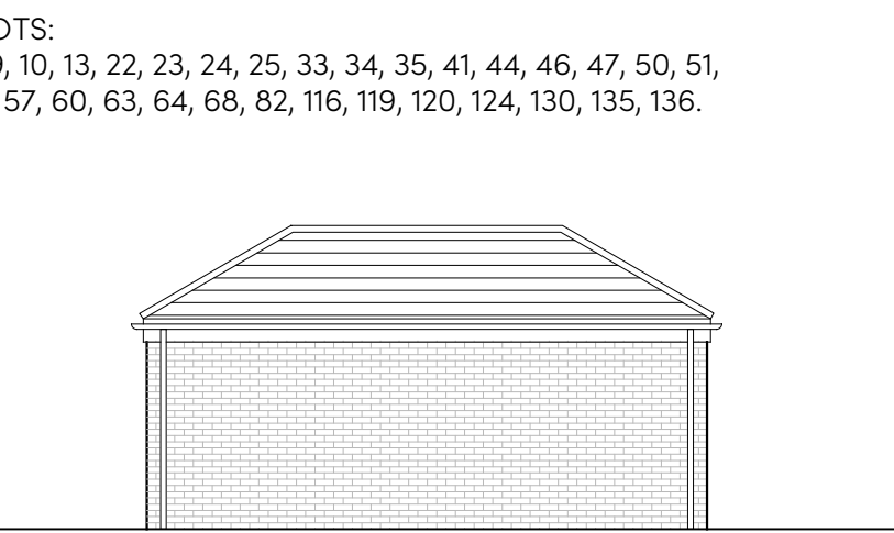
SIDE ELEVATION 1
