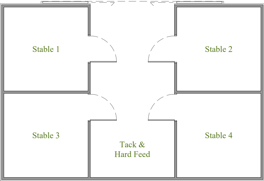
Ground Floor Plan 1:100 PROPOSED
