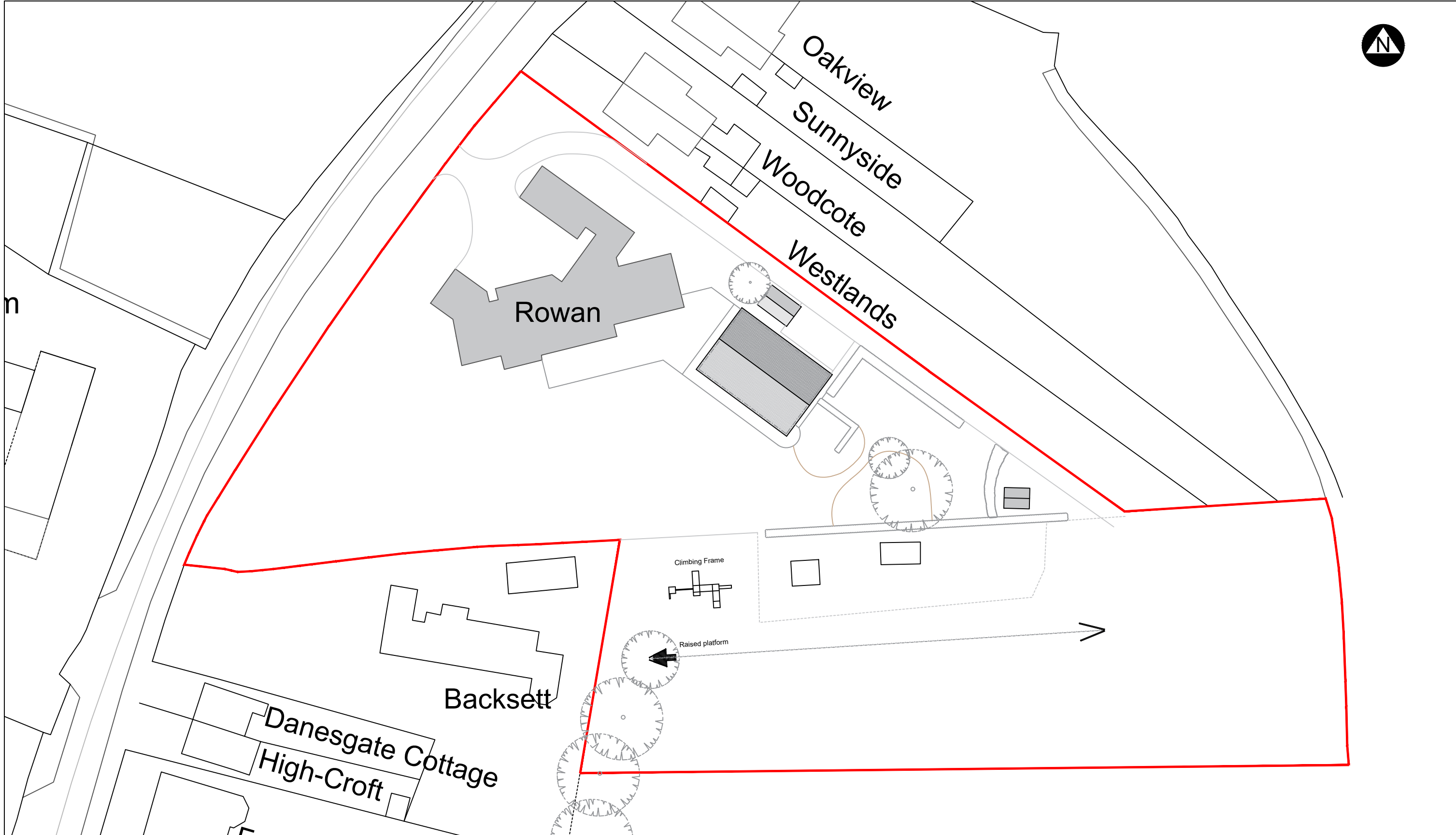
Existing block plan (Scale 1:500)
