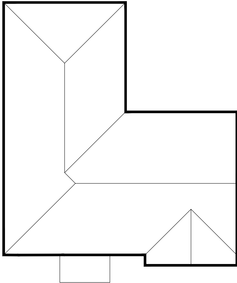
Roof Plan
