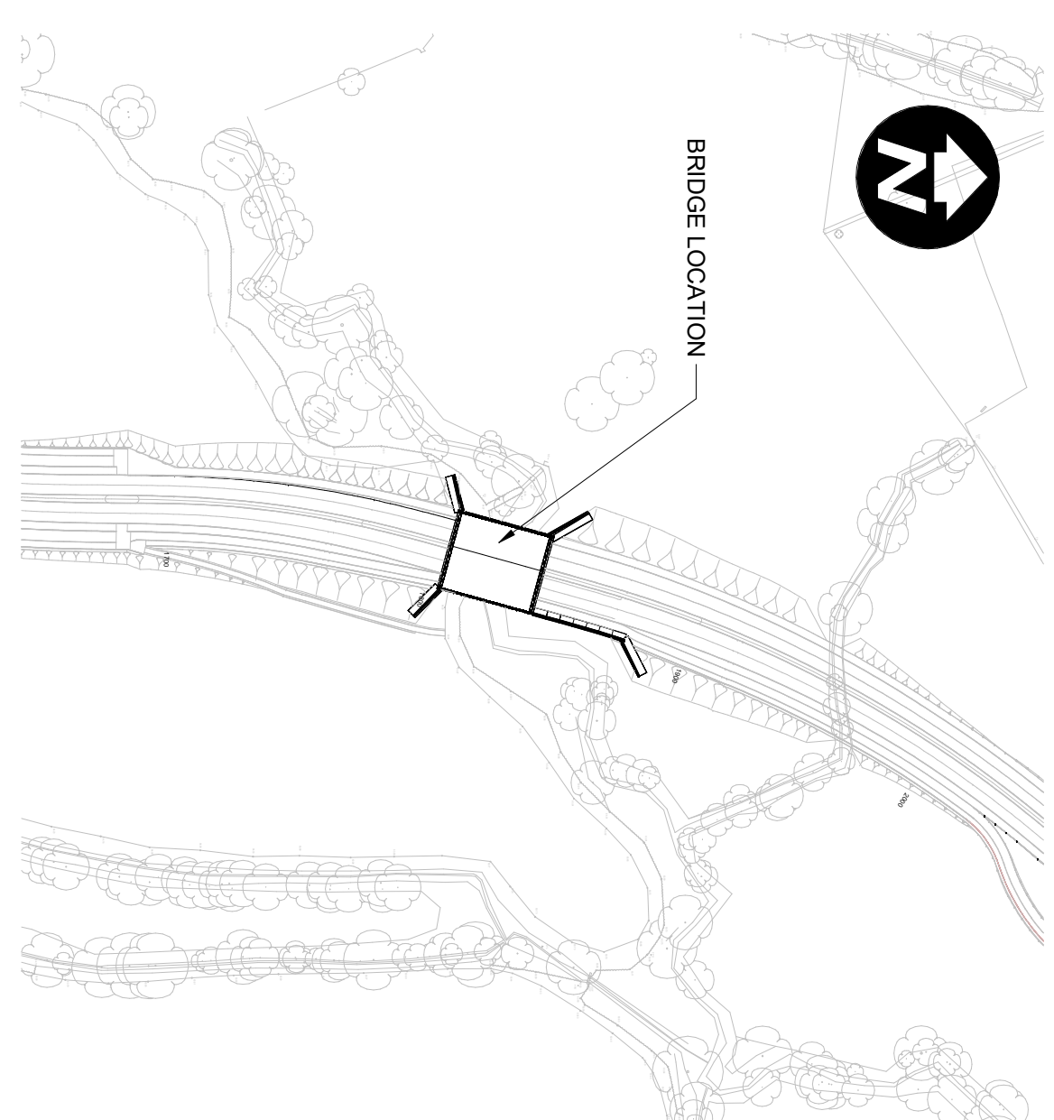
LOCATION PLAN 1 : 2500
