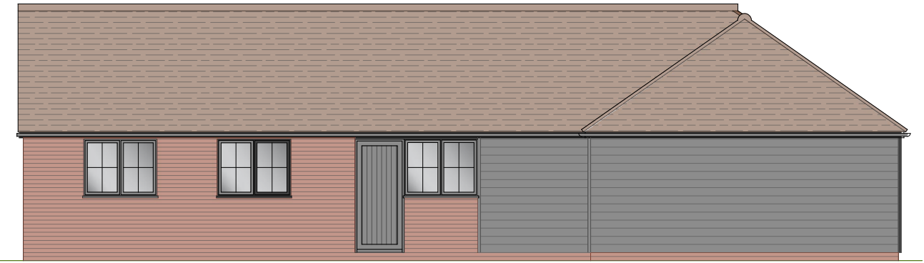
East 1:100 PROPOSED
