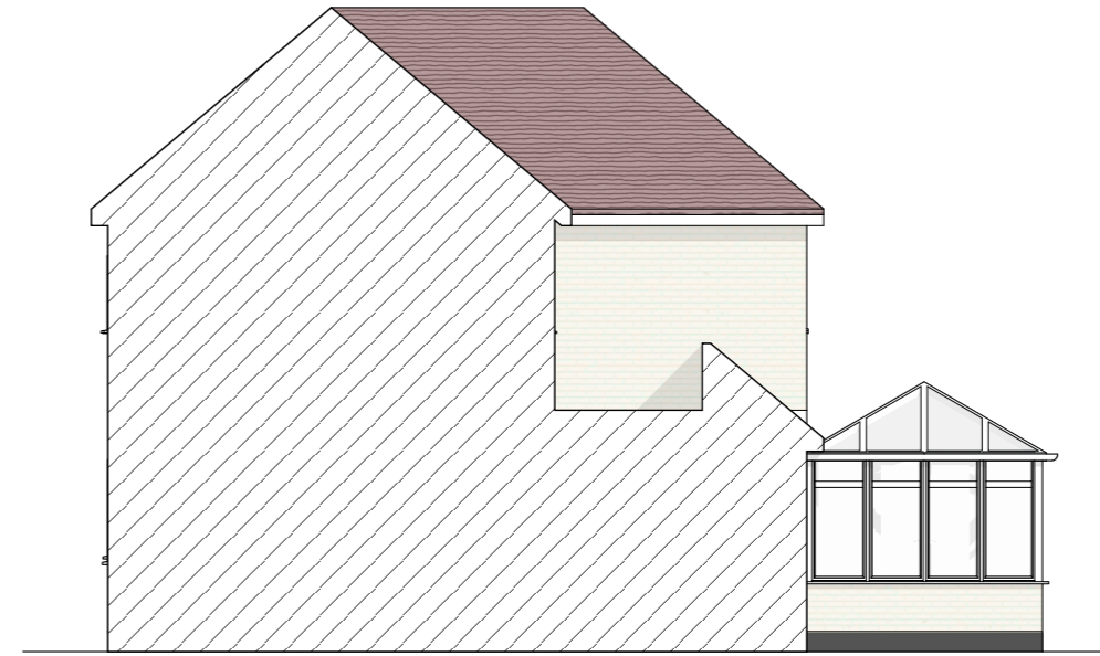
A :: Existing South East Elevation 04 scale: 1:100
