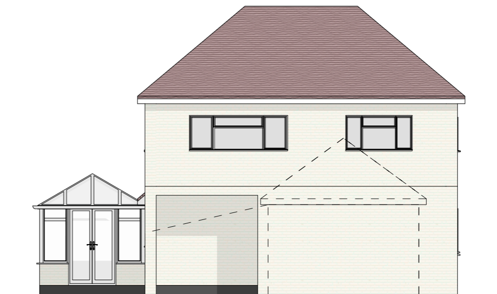
A :: Existing North West Elevation 04 scale: 1:100
