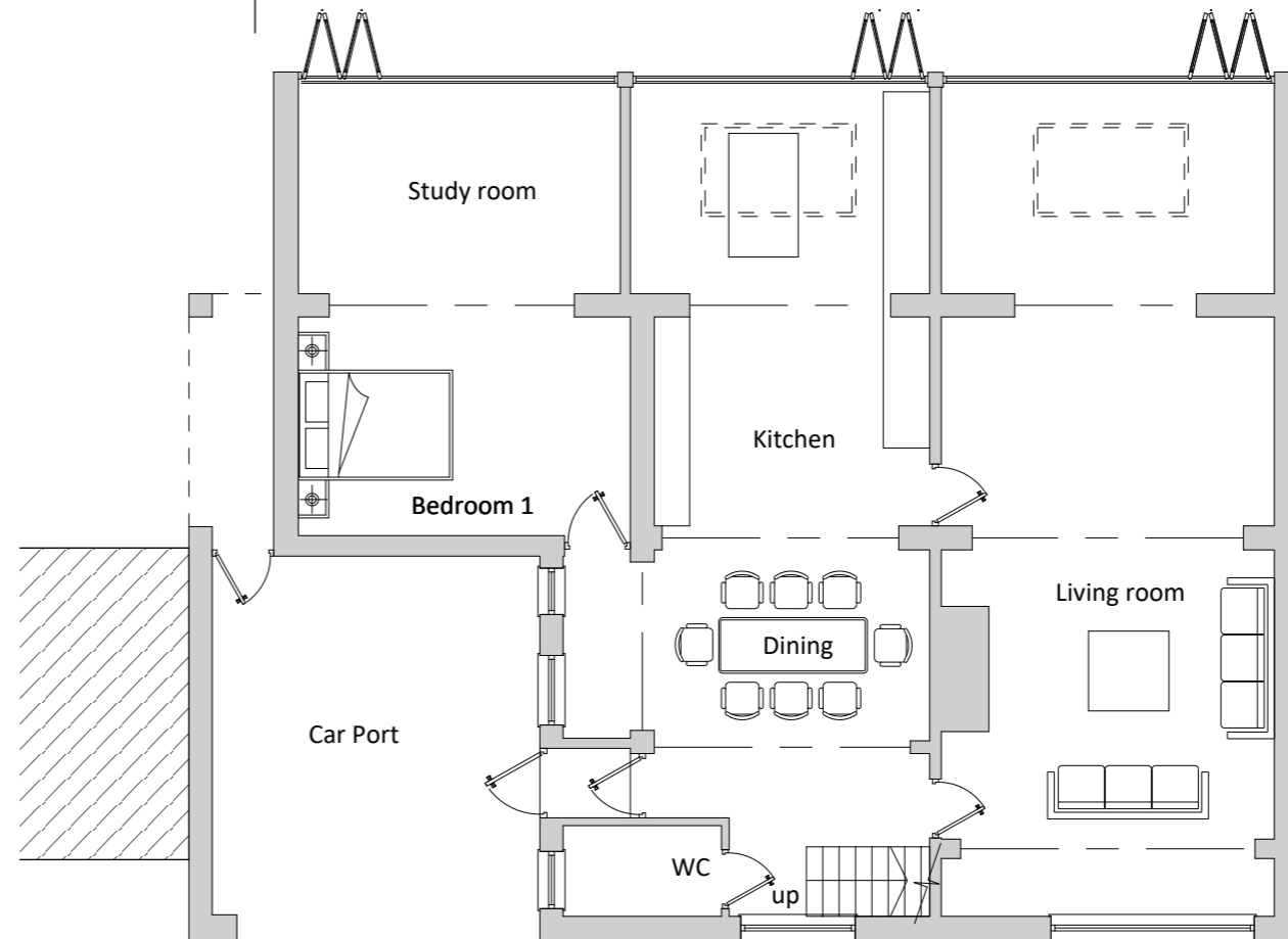
A :: Proposed Ground Floor Plan 02 scale: 1:100
