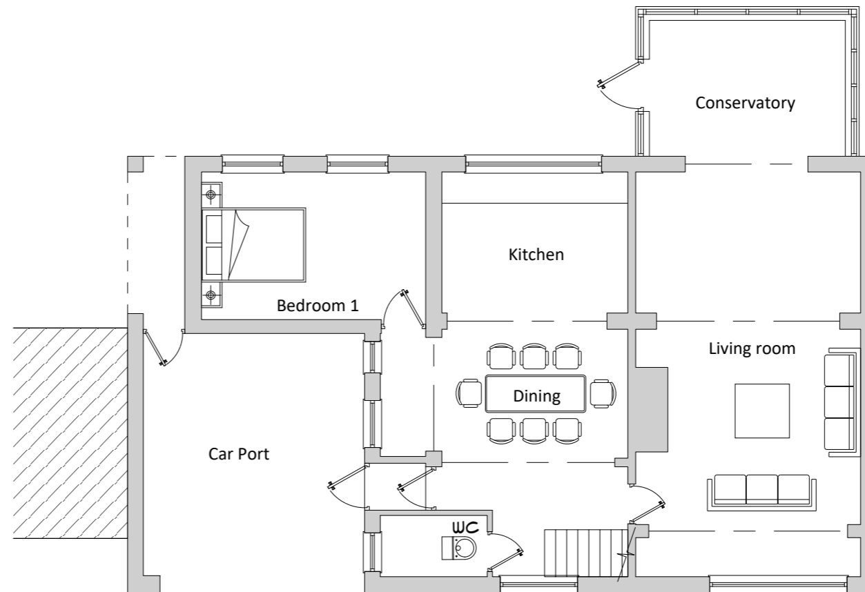
A :: Existing Ground Floor Plan 01 scale: 1:100
