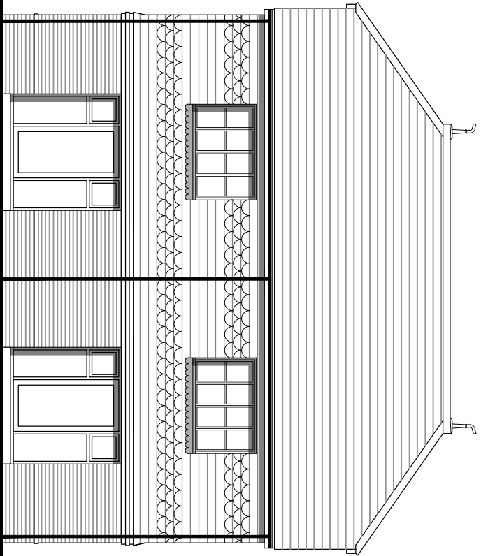
Rear Elevation
