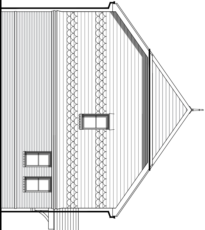
Side Elevation
